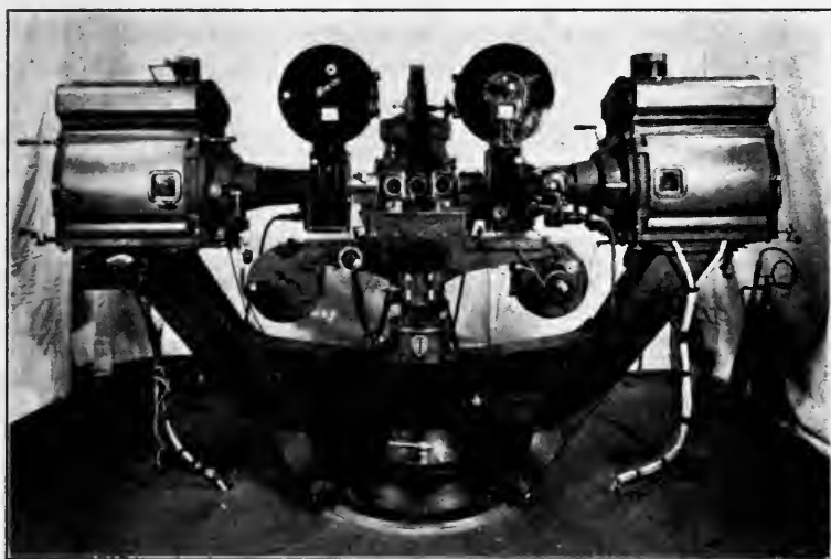
FIG. 5. Front view, showing division of lamp brackets from main base. The vertical load is carried on rollers in contact with the track forming the rim of the floor base. The projectors and optical bench are integral with the main rotating base.
